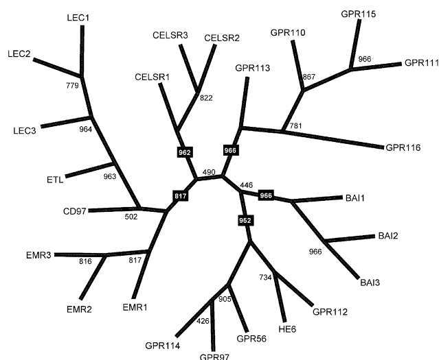
Fig. 2. Phylogenetic analysis of the new human GPCRs with other human LN-7TM receptors using the regions from TM1 to the end of TM7, obtained by maximum parsimony analysis (Phylip 3.6). The numbers above the nodes indicate percentage of bootstrap replicates. The accession numbers are listed in Table 1.
