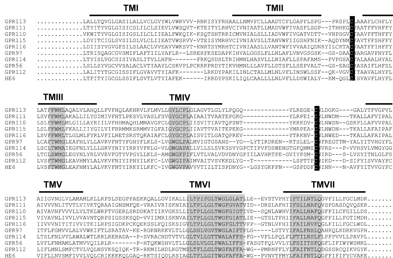
Fig. 1. Amino acid sequence alignment of the region from TM1 to TM7 of the novel human GPCRs, HE6 and GPR56 made using ClustalW (1.82) software and edited by manual inspection. The lines mark putative TM regions, and gray boxes indicate conserved sequence motifs. The accession numbers are listed in Table 1.
